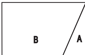
Fig. 9.3 Rectangle
