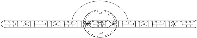
Fig. 4.5: Straight angle
