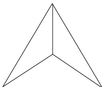
Fig. 12.7 (Pyramid with triangular base)
