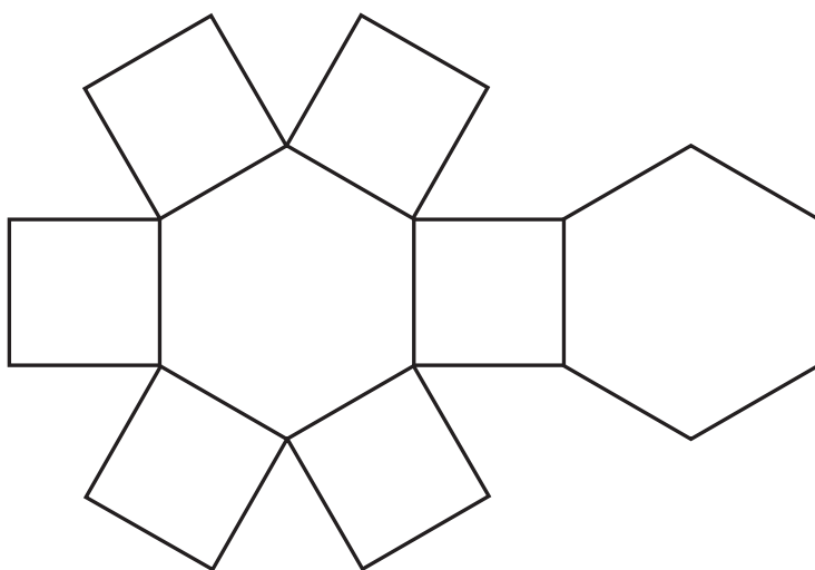
Net of Prism with Hexagonal base of Fig. 12.4
