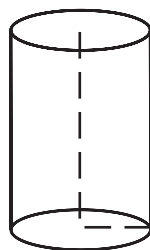
Fig. 12.2 (Cylinder)
