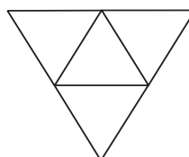
(i) Triangular base
