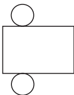
(e) Cylinder
