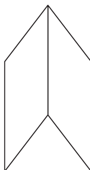
Fig. 12.6 (Prism with triangular base)
