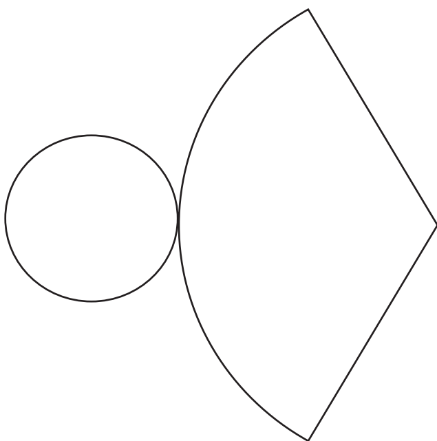
Net of Cone of Fig. 12.5
