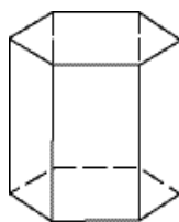
Fig. 12.4 (Hexagonal)
