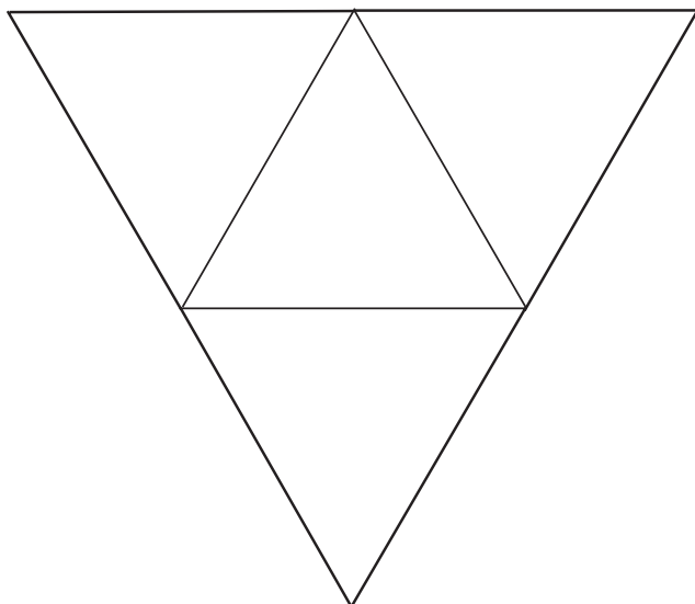
Net of Pyramid with Triangular base of Fig. 12.7
