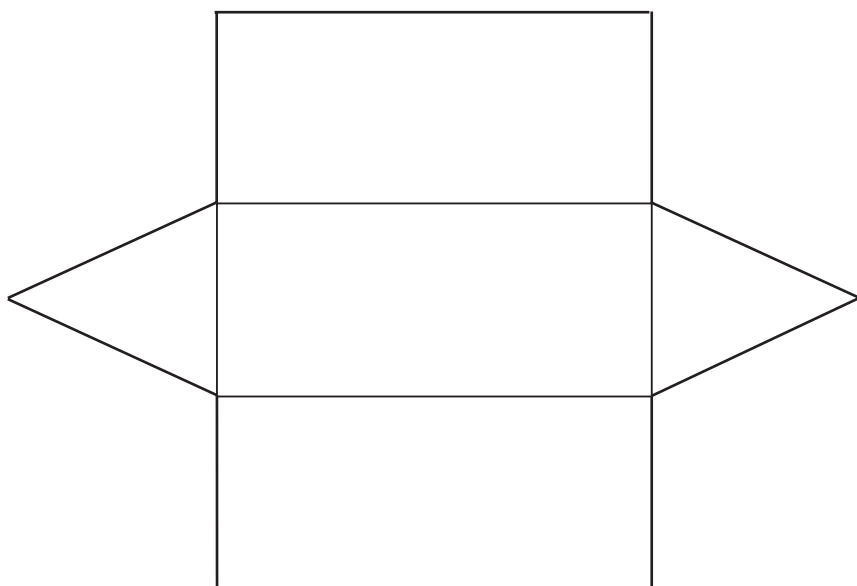
Net of Prism with Triangular base of Fig. 12.6
