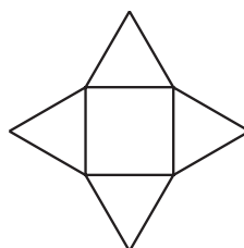
(ii) Square base
