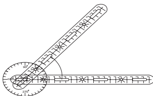
Fig. 4.2: Acute angle
