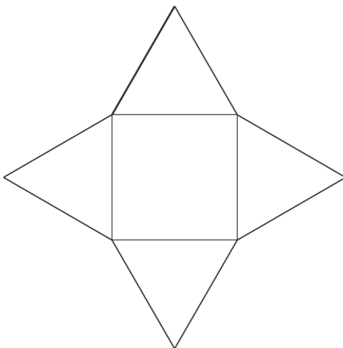
Net of Pyramid with Square base of Fig. 12.8
