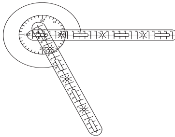
Fig. 4.6: Reflex angle
