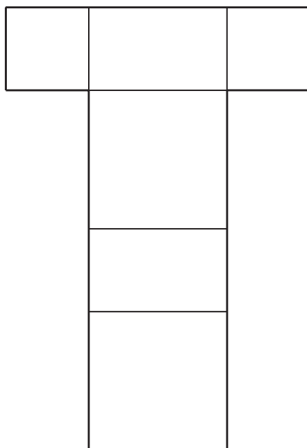
Net of Cuboid of Fig. 12.3
