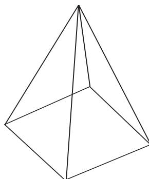
Fig. 12.8 (Pyramid with square base)
