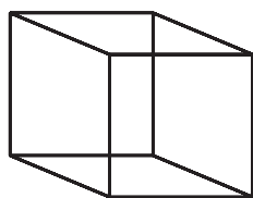
Fig. 12.1 (Cube)
