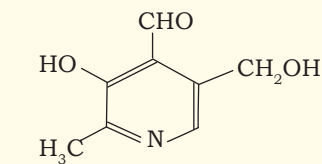
Pyridoxal (I)
