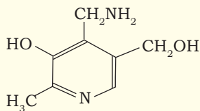
Pyridoxamine (III)
